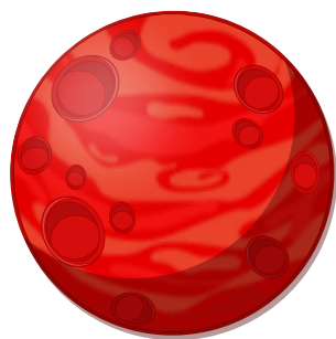
planets
